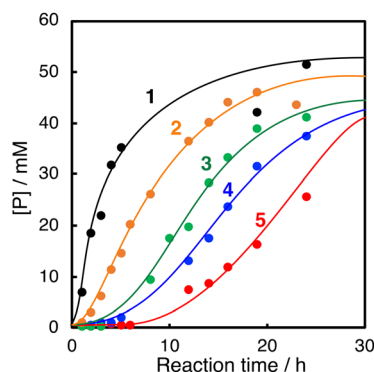
Fig. 3 Time courses of product formation in the oxidation of cyclohexane (2.0 M) catalysed by Cu II -complexes (1-5, 0.2 mM) with PhCHO (0.2 M) in CH 3 CN/CH 2 Cl 2 (v/v = 3/2) at 40 °C under O 2 . [P] = [A] + [K] + [L] + [CyCl]. Reduction potentials of the Cu II -complexes (vs. Fc/Fc + in acetonitrile) are shown in parentheses. The cyclic voltammograms of the Cu II -complexes are presented in Fig. S2†
