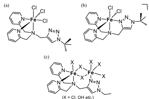
Fig. 2 Schematic drawings of the coordination structures of the iron(III) complexes. (a) [FeCl 2 L] (ref. 18), (b) [FeCl 2 L] 1+ (ref. 18), and (c) possible structures of the iron complex on the FeCl 3 -derived catalysts.
