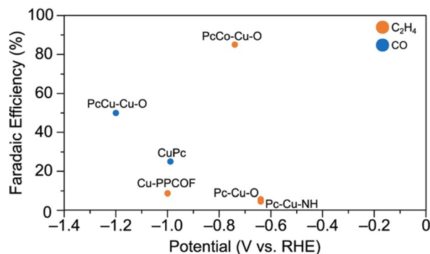
Fig. 10 Major \text{CO}_2\text{RR} product selectivity by metallophthalocyanine-based electrocatalysts. The data for PcCu-Cu-O are from Qiu et al. 113 The data for CuPc are from Kusama et al. 122 The data for PcCo-Cu-O, Pc-Cu-O, and Pc-Cu-NH are from Meng et al. 118 The data for Cu-PPCOF is from Zhang et al. 117 All data are reported for the conditions at which the highest single product FE is obtained.
