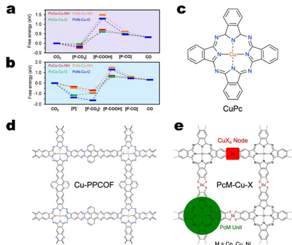
Fig. 9 Free energy diagrams for CO production on metallophthalocyanine-based Cu MOFs considering the a) concerted PCET mechanism and b) sequential PCET mechanism. Free energies are relative to desorbed \text{CO}_2 . Adapted with permission from Meng et al. 118 Copyright 2020 American Chemical Society. The structures of c) molecular PcCu, d) Cu-PPCOF, and e) Pcm-Cu-X.
