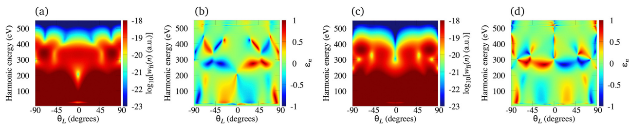
Fig. 7 Logarithm of the harmonic emission rate and the harmonic ellipticity of the N_2^+ cation for odd [panel (a) and (b)] and even [panel (c) and (d)] harmonics, obtained using the \omega - 2\omega OTC field with the relative phase \varphi = 0^\circ , as a function of the harmonic energy and the orientation angle \theta_L . The intensity of both field components is the same I = E_1^2 = E_2^2 = 10^{15} \text{ W cm}^{-2} , while the fundamental wavelength is 1300 nm.
