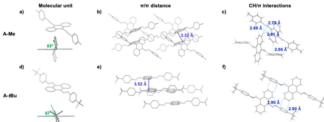
Fig. 3 Single crystal structures of (a)–(c) A-Me , and (d)–(f) A-tBu . Both crystals were grown through controlled release of the guests from their host-guest complexes with ExBox 4+ using guest displacement (GuD) via pyrene.
