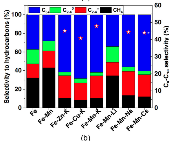
Fig. 16 Catalyst performance for the FT synthesis in terms of (a) the \text{CO}_2/\text{H}_2 conversion rate and (b) selectivity to hydrocarbons, especially longer-chain carbons (SAF). From ref. 102.
