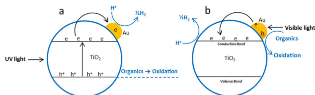
Fig. 12 Proposed photoreforming mechanism over \text{Au}/\text{TiO}_2 ; (a) under UV light irradiation (b) under visible light irradiation.
