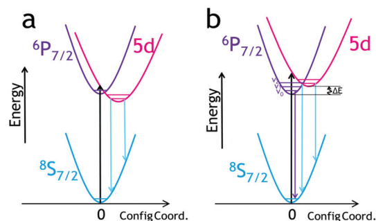
Fig. 1 Schematic diagram of the energy levels of the Eu 2+ ion. In (a), the 5d level is positioned below the 6 P 7/2 one, which precludes the 6 P 7/2 \rightarrow 8 S 7/2 radiative relaxation, and only the 5d \rightarrow 4f luminescence occurs. In (b), both narrow and broadbands corresponding to the 6 P 7/2 \rightarrow 8 S 7/2 and 5d \rightarrow 4f( 8 S 7/2 ) transitions, respectively, are possible, and their relative intensities (populations) are mainly governed by thermal coupling (situation valid for the SrB 4 O 7 :Eu 2+ system).
