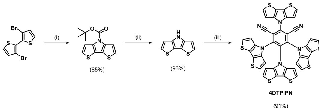
Scheme 1 Synthesis pathway toward 4DTPIP : (i) CuI, tert -butyl carbamate, N,N' -dimethylethylenediamine, K 2 CO 3 , toluene, 110 °C, 24 h; (ii) K 2 CO 3 , methanol, room temperature, 5 h; (iii) tetrafluoroisophthalonitrile, NaH, THF, 50 °C, 16 h.
