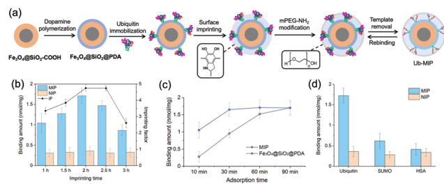
Fig. 3 (a) Schematic illustration of the construction of nano receptors for ubiquitin by surface imprinting over uniformly oriented templates on PDA preformed over silica coated magnetic nanoparticles (SiMNPs). (b) Binding amounts of ubiquitin on MIP and NIP NPs synthesized at different imprinting time and modified with mPEG-NH _2 at 25 mg mL ^{-1} . (c) Comparison of the binding kinetics of ubiquitin on MIP NPs and Fe _3\text{O}_4 @SiO _2 @PDA. (d) Selectivity test results of the MIP towards ubiquitin. The concentrations of MIP NPs and the tested proteins are 0.2 mg mL ^{-1} and 0.4 \mu\text{M} , respectively.
