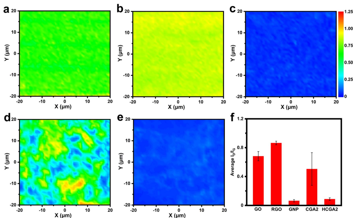
Fig. 3 Raman mappings of (a) GO, (b) RGO, (c) GNP, (d) CGA2, and (e) HCGA2. The blue, green, and red colors correspond to their I_D/I_G values of 0, ~0.6, and ~1.25, respectively. (f) Average I_D/I_G histograms of GO, RGO, GNP, CGA2 and HCGA2.
