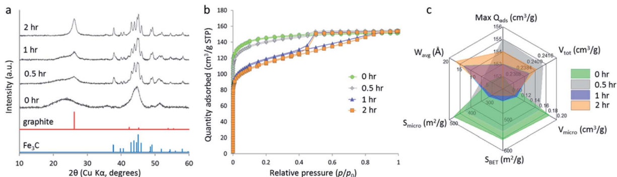
Fig. 9 (a) XRD data, (b) N 2 adsorption/desorption isotherms and (c) porosimetry data for carbons prepared by pyrolyzing starch and Fe(NO 3 ) 3 to 800 °C for various hold-times. Figure reproduced with permission from ref. 108.
