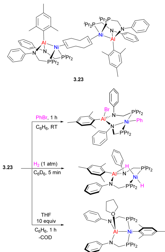
Scheme 23 Reactivity of (PAIP)Ni complex in oxidative addition and mesityl group transfer from Al to Ni.
