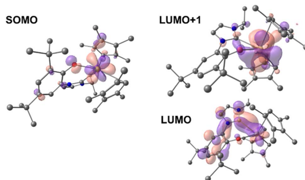
Fig. 3 Depictions of the TD-DFT-calculated SOMO (left) and LUMO+1 (right, upper) and LUMO (right, lower) orbitals of 1-Ce .
