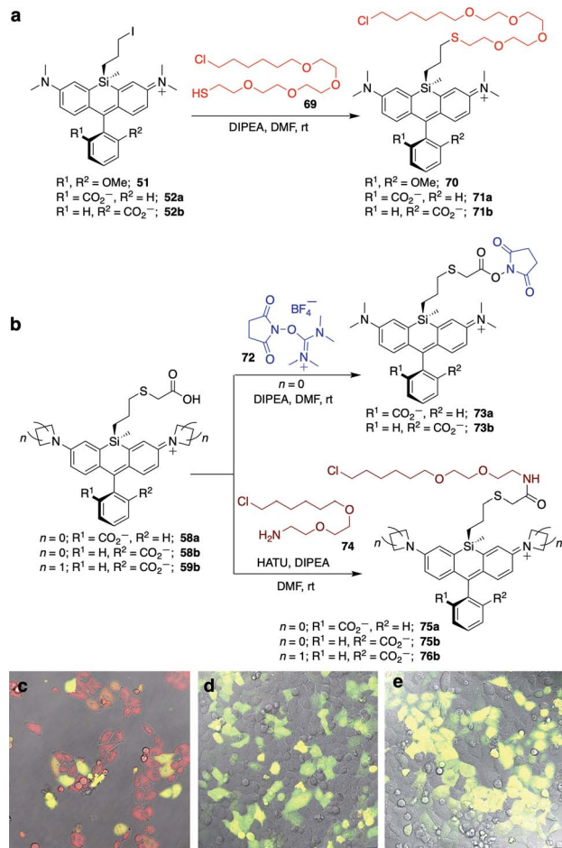
Fig. 3 Synthesis of Si-bridge NHS esters, HaloTag-ligand dyes, and no-wash live cell imaging in HeLa cells transfected with pHaloTag-EGFP. (a) Thio (O4) HaloTag ligand dyes 70 – 71b ; (b) Si-bridge NHS esters 73a – b and amine (O2) HaloTag ligand dyes 75a – 76b ; (c–e) Overlay of GFP, DIC, and dye fluorescence in cells treated with 200 nM (c) 75a ; (d) 75b ; (e) 76b . Scale bar is 20 \mu m.
