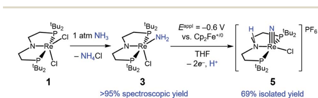
Scheme 7 Full conversion of NH 3 by 1 to a nitride in complex 5 .
