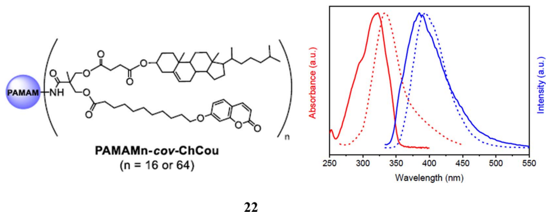
Fig. 15 Dendritic molecule of fluorescent coumarin moieties (22).
