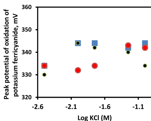
Fig. 6 Effect of concentration of KCl supporting electrolyte (3–100 mM) on the potential of three reference electrodes based on: mesoporous ceramic frit A (blue), mesoporous ceramic frit B (black), and commercially available free flow (red). Shown is the peak potential of the \text{Fe}(\text{CN})_6^{4-} (0.1 mM) oxidation as determined from CVs.
