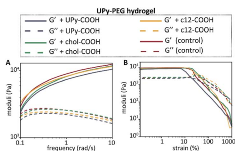
Fig. 4 Mechanical hydrogel properties of the BF UPy-PEG hydrogel upon anchor addition, with the frequency sweep at 1% strain (A), and the strain sweep at 1\ \text{rad s}^{-1} (B) measured at 37\ ^\circ\text{C} .
