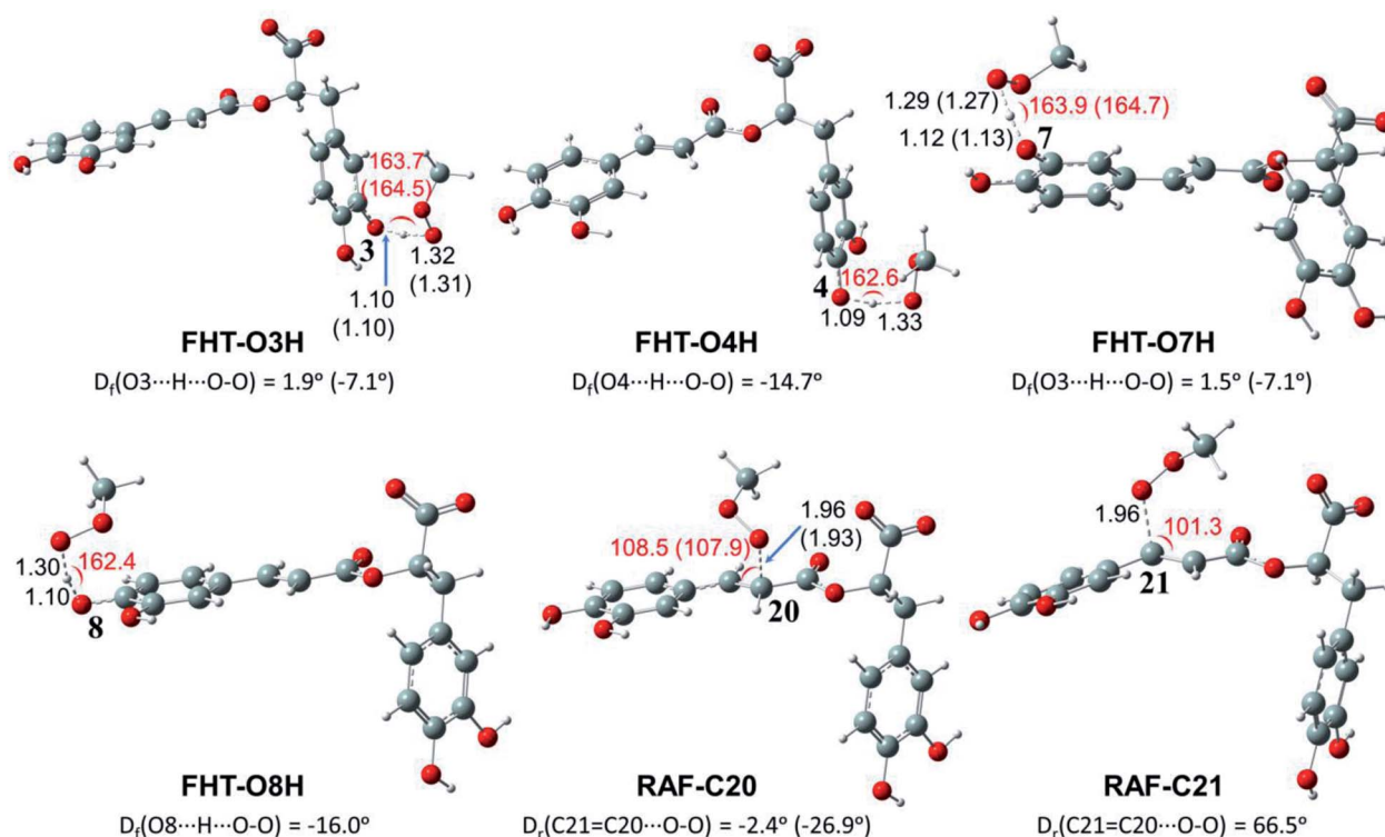
Fig. 4 Optimized structures of the transition states (TSs) for FHT and RAF reactions of rosmarinate mono-anion ( RA^- ) towards CH_3OO^* radicals in water calculated at the M05-2X/6-311++G(2df,2p) level of theory. D_f is the OHOO dihedral angle of the FHT TSs; D_r is the CCOO one of the RAF TSs. The values in parentheses correspond to the geometrical parameters obtained in the PEA phase.
