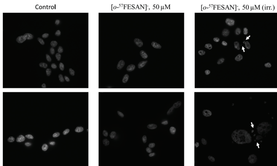
Fig. 11 Fluorescence microscopy for visualizing cellular responses in non-treated cells (control; left panel), 50 \mu\text{M Na}[o\text{-}^{57}\text{FESAN}] -treated but non-irradiated cell (middle panel), or 50 \mu\text{M Na}[o\text{-}^{57}\text{FESAN}] -treated cells that were also subjected to Mössbauer irradiation (right panel). Morphological damage to the nucleus was observed as indicated by the presence of nuclear fragments and abnormalities (white arrows).
