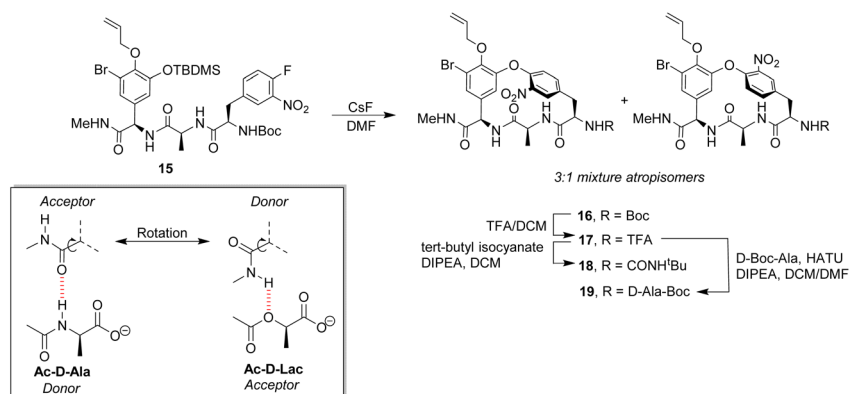
Scheme 2 CsF-induced \text{S}_{\text{N}}\text{Ar} macrocyclization of linear precursor 15 to biomimetic receptors 16–19 and schematic of methyl amide donor–acceptor H-bonding to Ac-D-Ala/Lac.
