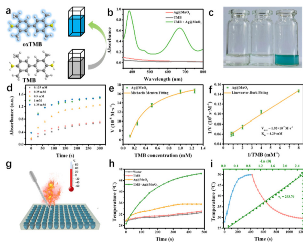
Fig. 3 Assessments of the oxidase-like activity and photothermal performance of Ag@MnO 2 : (a) schematic illustration of the oxidase-like catalytic process of Ag@MnO 2 nanozymes; (b) UV-Vis absorption spectra of Ag@MnO 2 , TMB, and [Ag@MnO 2 + TMB] in the 0.1 M PBS solutions (pH 6.0); (c) digital photographs of Ag@MnO 2 , TMB, and [Ag@MnO 2 + TMB] reaction solution; (d) time-dependent absorbance changes at 652 nm in [Ag@MnO 2 + TMB] with different TMB concentrations; (e) corresponding Michaelis–Menten curves and (f) Lineweaver–Burk plot of the Ag@MnO 2 nanoenzyme; (g) schematic illustration of the photothermal detection procedure of the [Ag@MnO 2 + TMB] reaction system; (h) temperature increasing profiles of water, Ag@MnO 2 , TMB, and [Ag@MnO 2 + TMB]; (i) linear time constant calculated from the cooling period in [Ag@MnO 2 + TMB].
