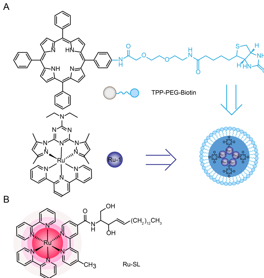
Fig. 20 (A) Structure of the lysosome-targeting nanoparticles \text{Ru-1@TPP-PEG-biotin} . 224 (B) Structure of the Golgi-targeting complex \text{Ru-SL} . 232
