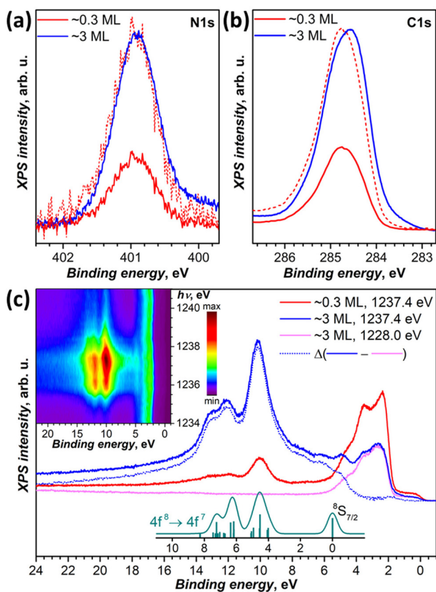
Fig. 4 (a and b) XPS spectra of \text{Tb}_2@C_{79}\text{N} on \text{Cu}(111) in the N 1s (a) and C 1s (b) energy range, measurements are performed at 77 K with excitation at 800 eV for submonolayer ( \sim 0.3 ML, red curves) and multilayer ( \sim 3 ML, blue curves); dashed red curves are spectra of the submonolayer sample scaled to match intensity of the multilayer. (c) Valence band photoelectron spectra with excitation at 1228 eV (off-resonance, magenta) and at 1237.4 eV (in resonance with 3d \rightarrow 4f excitation of Tb at the M_5 edge) compared to theoretical intensity of 4f^8 \rightarrow 4f^7 ionization transitions as calculated by Gerken 91 (cyan, vertical bars are individual transition, and the curve is Gaussian broadening with the peak width of 0.6 eV). Blue dotted curve is the difference between in-resonance and off-resonance spectra. The inset shows variation of the PES intensity with the excitation photon energy between 1234 and 1241 eV measured with the step of 0.2 eV.
