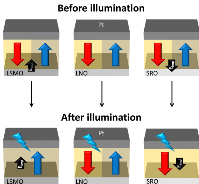
Fig. 5 Sketch of the direction of E_{\text{imp}} in the different studied samples. The effect of light on the polarization results in its switching towards the E_{\text{imp}} direction.
