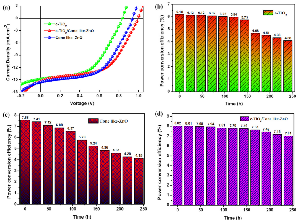
Fig. 8 Use of cone-like ZnO improves the perovskite solar cell performance. (a) Better J-V characteristics of upon addition of the cone-like ZnO as a part of ETL. (b–d) PCE over time for the single layer \text{c-TiO}_2 , cone-like ZnO and bilayer of \text{c-TiO}_2 with cone like ZnO as ETL. Reprinted with permission from ref. 180. Copyright 2021 Springer Nature.
