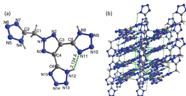
Fig. 7 (a) Thermal ellipsoid plot (50%) and labeling scheme for 7 . (b) A ab axis view of the ball-and-stick packing diagram of 7 .
