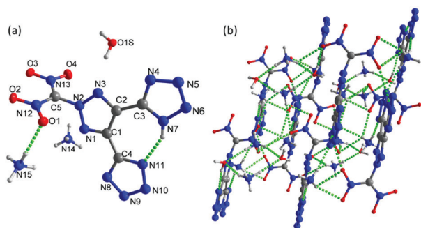
Fig. 5 (a) Thermal ellipsoid plot (50%) and labeling scheme for 5a-H 2 O . (b) A ab axis view of the ball-and-stick packing diagram of 5a-H 2 O .
