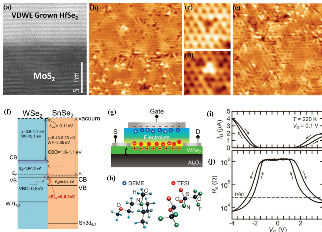
Fig. 2 (a) HAADF-STEM image of \text{HfSe}_2 grown on \text{MoS}_2 by MBE. The figure has been reproduced from ref. 82. (b) STM micrograph of \text{TiSe}_2 thin film ( 17 \text{ nm} \times 17 \text{ nm} , I = 100 \text{ pA} , and V_s = 0.24 \text{ V} ), showing the two kinds of Se defects: bright Se interstitials and dark Se vacancies. Zoomed-in STM micrographs of a single (c) Se vacancy and (d) interstitial ( 2 \text{ nm} \times 2 \text{ nm} , I = 100 \text{ pA} , and V_s = 0.24 \text{ V} ). (e) STM micrograph of a charge density waves (CDW)-related 2 \times 2 superstructure in single-layer \text{TiSe}_2 thin film ( 20 \text{ nm} \times 20 \text{ nm} , I = 100 \text{ pA} , and V_s = 0.1 \text{ V} ). The figures have been reproduced from ref. 83. (f) Schematic of the band alignment at the \text{WSe}_2/\text{SnSe}_2 heterojunction as revealed by X-ray photoelectron spectroscopy (XPS) core level analysis. E_F and \chi denote the Fermi energy and electron affinity, respectively. E_g is the band gap, whereas VBO and CBO denote the valence and conduction band offsets, respectively. The figure has been reproduced from ref. 84. (g) Schematic of the top-gated electric-double-layer transistor (EDLT) based on the \text{WSe}_2 epitaxial thin film grown on the sapphire substrate. (h) Chemical structure of the electrolyte used in the electrolyte-gated transistor. (i and j) show typical transfer characteristics of \text{WSe}_2 -EDLT carried out at T = 220 \text{ K} , indicating clear ambipolar operation. The figures have been reproduced from ref. 79.
