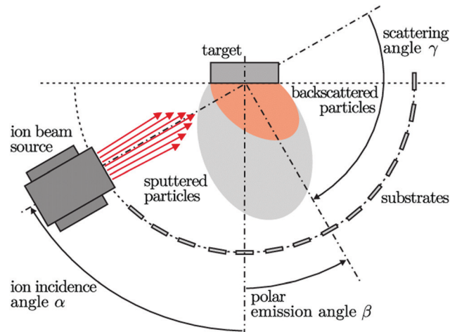
Fig. 19 Representation of the ion-beam sputtering system.
