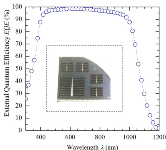
Fig. 4 External quantum efficiency (EQE) curve of the best solar cell, in which the EQE beam spot was centered within the metallic fingers ( i.e. , active device area). Inset: Photograph showing solar cells of 1 \times 1 and 2 \times 2 cm 2 configurations. IV curve and power output characteristics of the champion solar cell.
