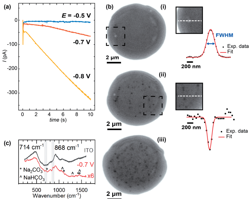
Fig. 5 (a) SECCM current and (b) IRM images for the electrochemically-induced precipitation of \text{CaCO}_3 at different applied potentials with a ca. 8\text{ }\mu\text{m} diameter SECCM meniscus. Applied potentials, E , (i) -0.5 V, (ii) -0.7 V and (iii) -0.8 V. Insets of b(i) and b(ii) show optical intensity line profiles of typical bright and dark features respectively, along with the corresponding Gaussian fits. IRM images recorded at 50 FPS and shown at the end of the potential pulse (10 s). Light source: blue LED (wavelength of 470 nm). (c) Raman spectrum from a dried meniscus deposited at -0.7 V (with the spectrum from bare ITO subtracted). The bare ITO spectrum is also shown.
