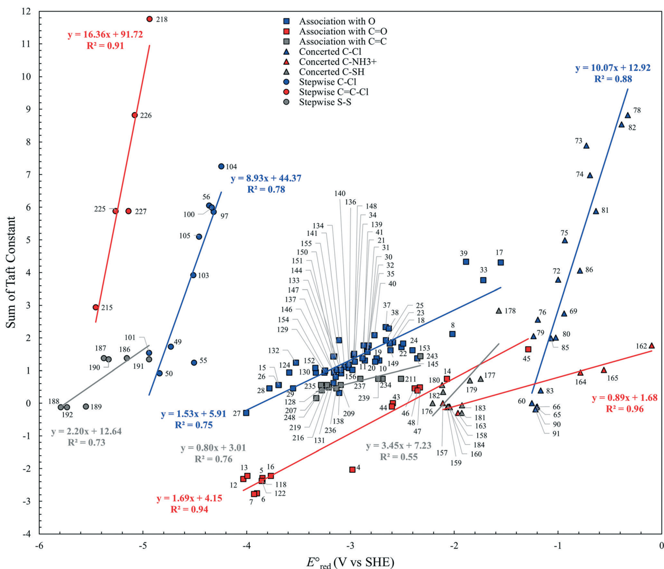
Fig. 3 Sum of Taft constants against the theoretically calculated E_{\text{red, aq}}^{\circ} values of each compound.
