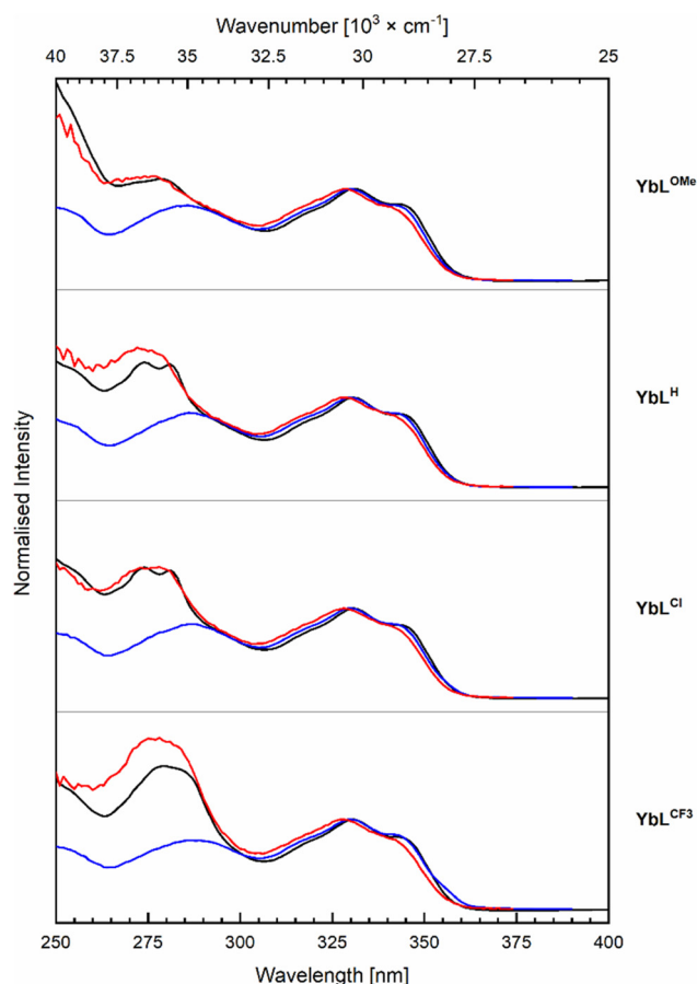
Fig. 5 Normalised excitation spectra for the Yb (red, \lambda_{\text{em}} = 978 nm) and antenna (blue, \lambda_{\text{em}} = 405 nm) emission with corresponding absorption (black) spectra of YbL X complexes. Recorded in PIPES buffered (10 mM, pH 6.5, A = 0.10 ) aqueous solutions at r.t.
