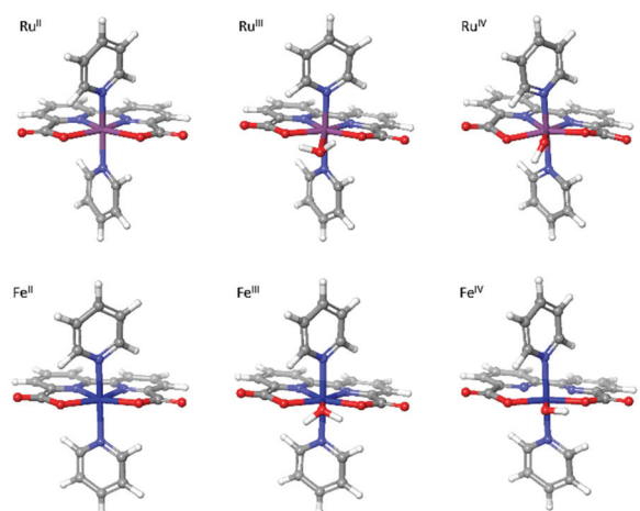
Fig. 2 Structures of \text{Ru}(\text{bda})(\text{py})_2 and \text{Fe}(\text{bda})(\text{py})_2 at \text{M}^{\text{II}} , \text{M}^{\text{III}} , \text{M}^{\text{IV}} states.
