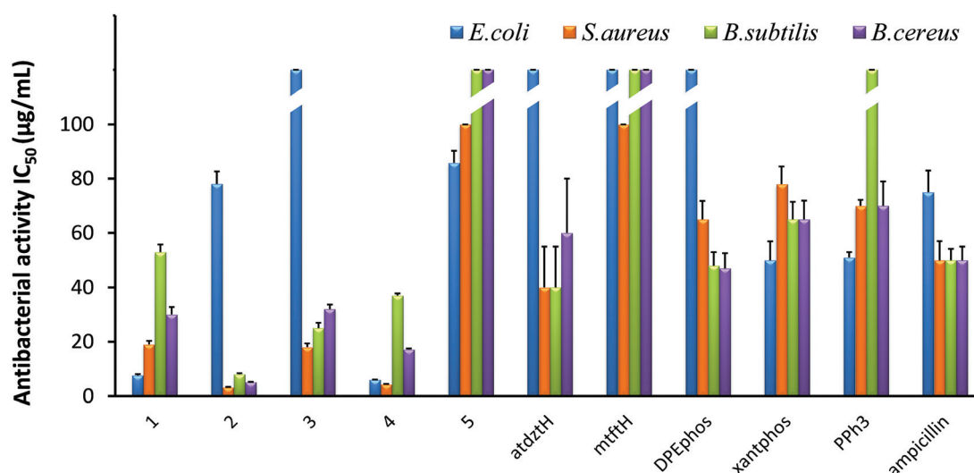
Fig. 3 In vitro antibacterial activity of 1–5 , and their ligands atdztH, mtftH, DPEphos, xantphos, and \text{PPh}_3 in free form, expressed as half-minimum inhibitory concentration ( \text{IC}_{50} ) values ( \mu\text{g mL}^{-1} ) provided by a nonlinear curve fit-growth/sigmoidal-dose response on the experimental optical density data. Values are expressed as mean \pm standard deviation (SD) of three replicate measurements (with the exception of values higher than 100 \mu\text{g mL}^{-1} ).
