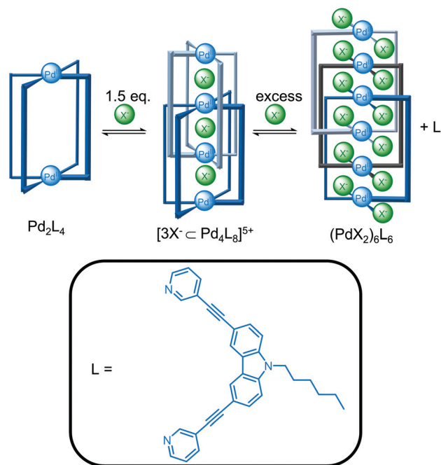
Fig. 3 Clever and co-workers' halide templated formation of a [\text{3X}^- \cdot \text{Pd}_4\text{L}_8]^{5+} interpenetrated double cage from a [\text{Pd}_2\text{L}_4](\text{BF}_4)_4 cage and subsequent conversion to the triply catenated (\text{PdX}_2)_6\text{L}_6 upon addition of excess halide ions.
