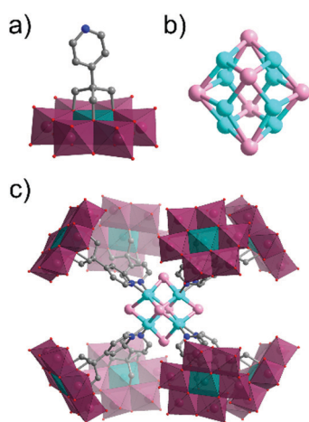
Fig. 7 Structure of the monotopic Anderson-Evans-type metal halide cluster, highlighting: (a) the {CrMo 6 } hybrid POM building block ({CrO 6 } = teal green octahedra); (b) the Cu 8 I 6 metal halide core and; (c) the assembled octameric nanostructure. This figure has been adapted from ref. 91 with permission from the American Chemical Society, copyright 2016.
