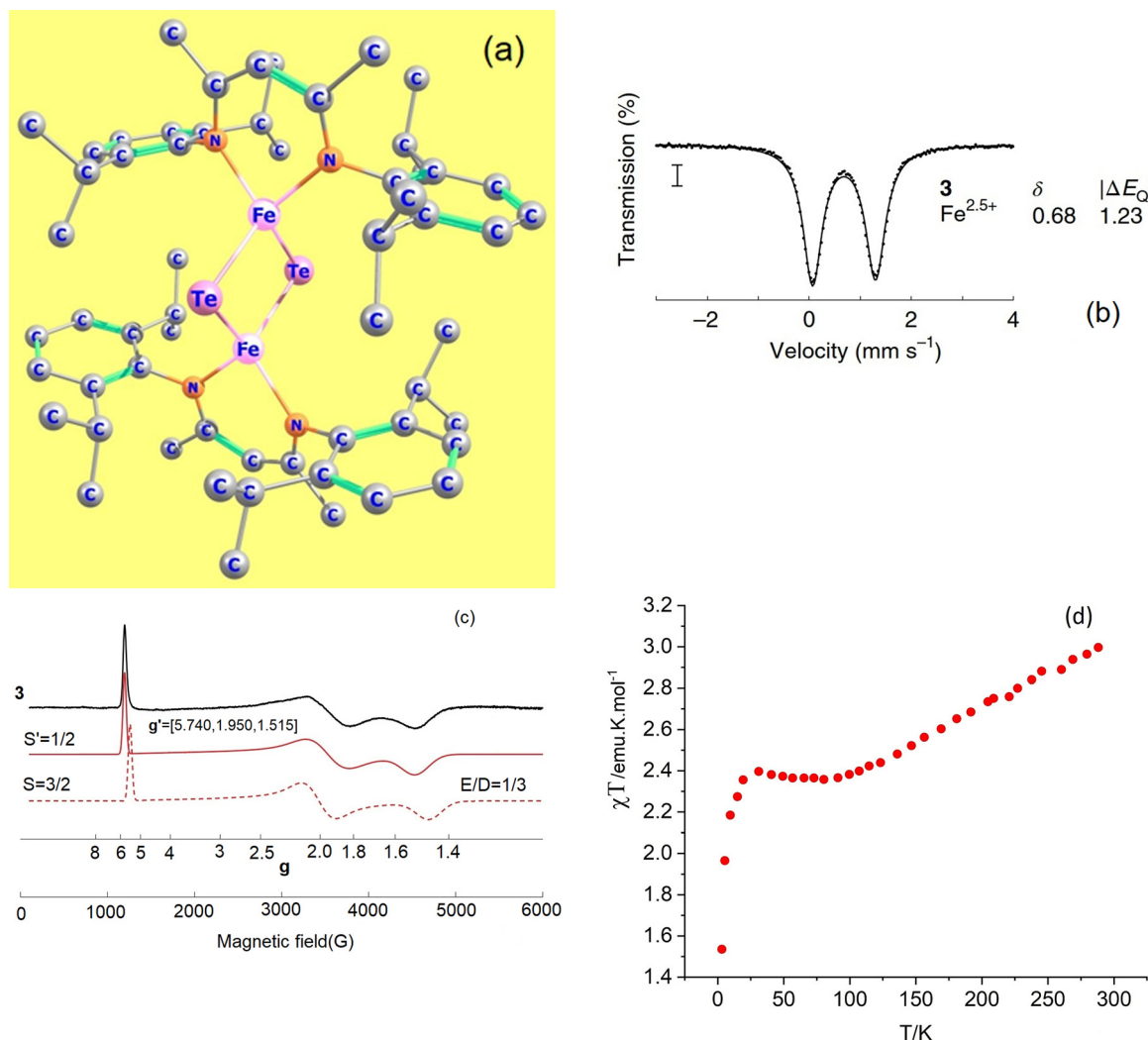
Fig. 2 Experimental X-ray structure of the mixed valence complex \text{Fe}^{2.5+}_{2}\mu_{2}\text{Te}_{2}\text{Fe}^{2.5+} (a); its T = 80 K Mössbauer spectrum in zero magnetic field (b); continuous-wave X-band EPR spectrum (9.63 GHz) of a frozen solution at 3.6–8 K, collected under non-saturating microwave power conditions (black line) and simulations (red lines): pseudo-spin S' = 1/2 , g' = 5.740, 1.950, 1.515 (solid red line) and a S = 3/2 , spin-Hamiltonian, |D| \gg h\nu , |E/D| = 1/3 (assuming g = g_e = 2.0023 ) and a value of D < 15 \text{ cm}^{-1} , estimated from the temperature dependence of the Lorentzian linewidth (c), variable-temperature SQUID magnetic susceptibility of a solid sample (d); data have been reproduced in a modified form from J. T. Henthorn, G. E. Cutsail III, T. Weyhermüller and S. DeBeer, "Stabilization of intermediate spin-states in mixed-valence diiron dichalcogenide complexes", Nat. Chem. , https://doi.org/10.1038/s41557-021-00853-5 .
