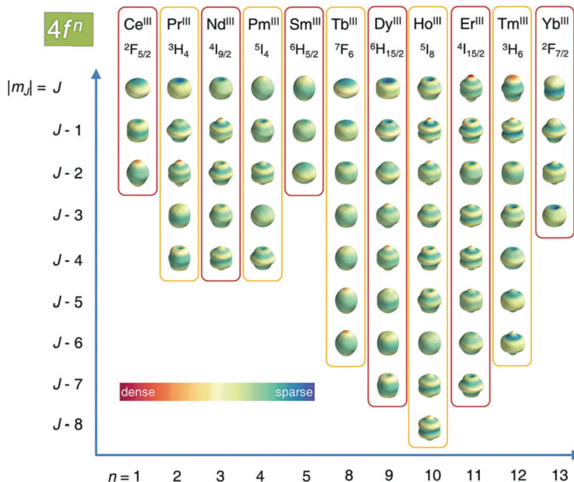
Fig. 5 Charge density angular distribution for lanthanoid(III) 4f shells for the different m_J states. Reproduced from ref. 66 with permission from the Royal Society of Chemistry.
