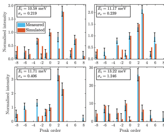
Fig. 4 Comparison of the measured (blue bars, see text for details) and the simulated peak intensities (orange bars) for the diffraction peaks along \overline{\Gamma Y} handed to the optimisation routines (see Fig. 5 for comparison). The error bars of the measurements were calculated with eqn (9).
