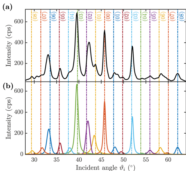
Fig. 3 (a) Characteristic \theta -scan of the Bi(114) surface along \overline{\Gamma Y} (measured data shown by the black line) with the sample temperature kept constant at T_s = 114 K. The energy of the incident helium beam was held constant at E_i = 10.58 meV. The coloured vertical lines represent the theoretically calculated peak positions with the corresponding \mathbf{G} -vectors. (b) Fits of the measured diffraction peaks using a scaled pseudo-Voigt profile.
