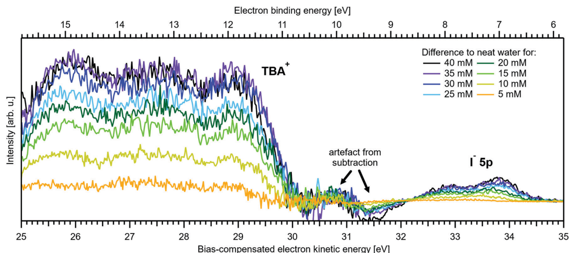
Fig. 7 Difference between the neat water spectrum and spectra for various concentrations of TBAI (aq) after normalization to the same 1\text{b}_1 peak height, i.e., it is assumed that solute contributions below the 1\text{b}_1 peak are zero. The reference spectrum (not shown, see red curve in Fig. 5B and Fig. S4, ESI†) has also been successively Gaussian-broadened before calculating the difference to account for the broadening effect observed with higher TBAI concentration (compare to the 1\text{b}_1 FWHM in Table 2). The signal contribution at an eKE of 25–30 eV is assigned to \text{TBA}^+ and increases in intensity similarly to the \text{I}^- 5\text{p} signal at 32–35 eV (see Fig. 6C).
