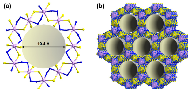
Fig. 8 Detail (a) and overall representation (b) of the crystal structure of [\text{Mn}_5\text{S}_{12}(\text{N}_2\text{H}_4)_6]\cdot(\text{H}_2\text{en})\cdot\text{DMF}\cdot 0.5\text{N}_2\text{H}_4 with 1D channels running along the crystallographic c -axis. Counterions are omitted for clarity. Color code: Sb-violet, Mn-lavender, S-yellow, N-blue.
