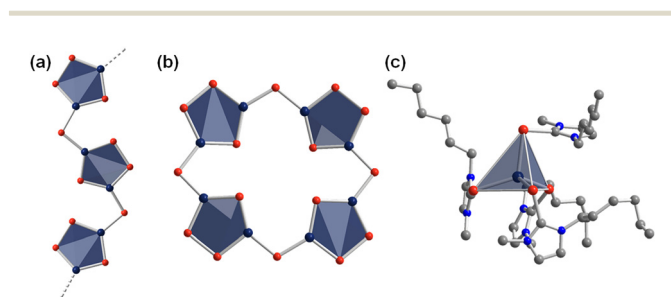
Fig. 3 Infinite zig-zag-strand structure of the anion 1\text{D}-[\text{Hg}_2\text{Te}_4]^{2-} (a), molecular structure of the heavy metal porphyranoid anion [\text{Hg}_8\text{Te}_{16}]^{8-} (b), molecular structure of the cationic complex [(\text{C}_6\text{C}_1\text{ImTe})_4\text{Hg}]^{2+} (c). Hydrogen atoms are omitted for clarity. Color code: Hg-dark blue, Te-red, C-grey, N-blue.
