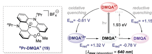
Scheme 10 Photophysical properties and redox potentials (vs. SCE in MeCN) of "Pr-DMQA + (ref. 43a).
