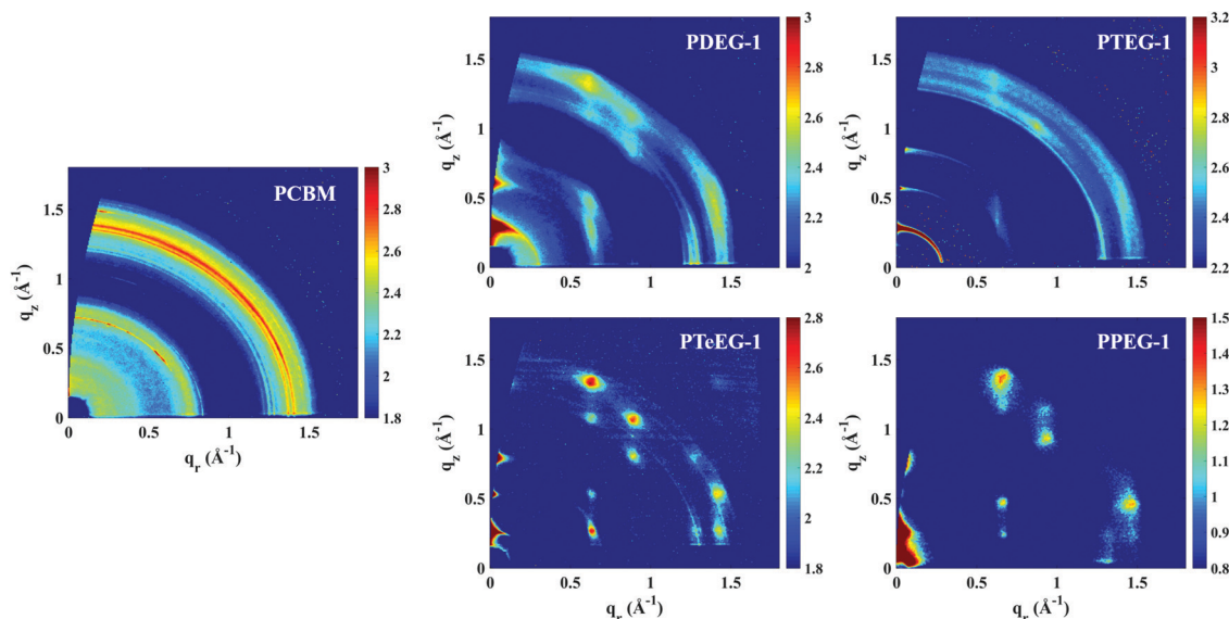
Fig. 2 GIWAXS patterns for the C 60 –EG derivatives spin coated from chloroform solutions. The GIWAXS for a PCBM thin film is also reported for comparison. Note that the PTEG-1 sample was measured using the lab X-ray instrument, while all the others were measured at the synchrotron.
