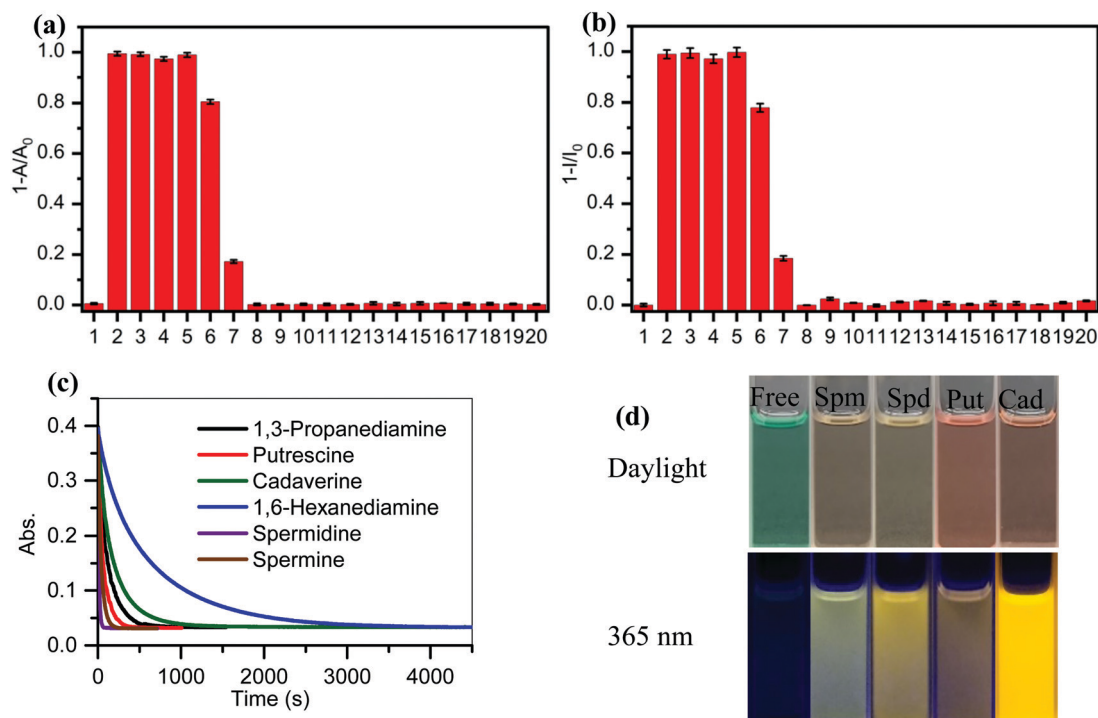
Fig. 3 (a) The absorption at 695 nm and (b) fluorescence changes at 720 nm of PPCy-1 (2.5 \mu\text{M} ) at 25 °C upon the addition of 50 \mu\text{M} of various amines for 2 min (1: blank, 2: spermine, 3: spermidine, 4: 1,3-propanediamine, 5: putrescine, 6: cadaverine, 7: 1,6-hexanediamine, 8: n -propylamine, 9: n -butylamine, 10: n -pentamine, 11: n -hexylamine, 12: n -heptylamine, 13: n -octylamine, 14: cyclohexylamine, 15: aniline, 16: p -methoxyaniline, 17: p -nitroaniline, 18: trimethylamine, 19: triethylamine, and 20: diethylamine). A_0 and A represent the absorption of PPCy-1 at 695 nm in the absence and presence of amine, respectively. I_0 and I represent the emission of PPCy-1 at 720 nm in the absence and presence of amine, respectively. (c) UV-vis kinetics for PPCy-1 with different BAs at 25 °C at a monitoring wavelength of 690 nm. (d) The photos of PPCy-1 in presence of spermine (Spm), spermidine (Spd), putrescine (Put) and cadaverine (Cad) on daylight and 365 nm irradiation.
