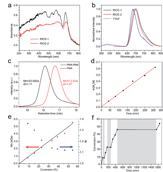
Fig. 3 (a). Solid-state UV-vis spectra of the RICE COFs (b). Fluorescence emission spectra of RICE COFs and TTAP monomer in DMF. Excitation wavelength 460 nm. (c). GPC profiles of PMA and the diblock copolymer (d) first order kinetic plot of the polymerization of MA (DP = 100) (e) M n and D of resulting polymers versus monomer conversion. Black line is theoretical M n vs. conversion. Blue dots are D at different conversion. Red dots are M n at different conversion. (f) Pulsed-irradiation kinetic experiments. The shaded areas indicate the reaction operated in the dark while the unshaded areas represent the reaction under irradiation.
