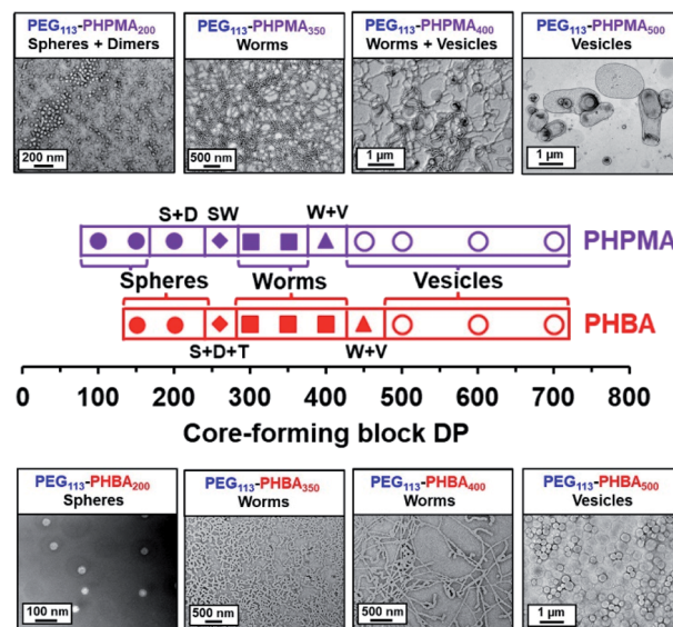
Fig. 3 Representative TEM images recorded for two series of PEG 113 -PHBA x and PEG 113 -PHPMA y diblock copolymer nano-objects prepared via RAFT aqueous dispersion polymerization of either HBA or HPMA at 30 °C when targeting 15% w/w solids. For the PEG 113 -PHBA x nano-objects, TEM studies required covalent stabilization using a GA crosslinker at 20 °C. Spheres, dimers, trimers, short worms, and worm plus vesicle mixed phases are denoted by S, D, T, SW and W + V, respectively.
