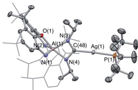
Fig. 4 Molecular structure of 5-Ag in the solid state as determined by X-ray crystallography. Thermal ellipsoids set at the 50% probability level. Hydrogen atoms omitted and ^1\text{Pr}/^1\text{Bu} shown in wireframe for clarity. Key bond lengths (Å) and angles ( ^\circ ): \text{Ag}(1)\text{--C}(48) : 2.118(2), \text{Ag}(1)\text{--P}(1) : 2.3851(6), \text{N}(3)\text{--C}(48) : 1.346(3), \text{N}(4)\text{--C}(48) : 1.345(3).
