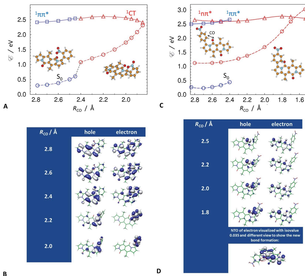
Fig. 9 Potential-energy profiles (PEPs) along the carbon–oxygen distances, R_{CO} , and the corresponding S_1 \rightarrow S_0 NTOs (isovalue = 0.03, unless indicated otherwise) optimized with the ADC(2)/def-SV(P) method in the lowest excited singlet states of (A and B) 5 and (C and D) 3. (A and C) Circles connected by dashed line denote vertical energy of the ground state computed at the geometry of the respective excited state. For 5, (A) locally-excited, ^1\pi\pi^* , state – blue squares, and the dark charge-transfer, ^1CT , state – red triangles; and (B) NTOs along R_{CO} . For 3, (C) locally-excited, ^1\pi\pi^* , state – blue squares, and the dark ^1n\pi^* state – red triangles; and (D) NTOs along R_{CO} , where the last bottom structure depicts the electron NTO at isovalue of 0.035 to visualize the formation of the carbon–oxygen covalent bond, as circled with a red dashed line.
